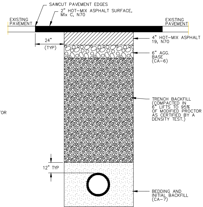
OPEN CUT FINAL STREET RESTORATION (CLASS D PATCH, 4")
