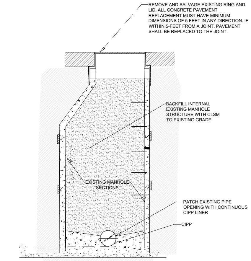
STANDARD MANHOLE DECOMMISSION DETAIL (PAVED SURFACE) NOT TO SCALE
