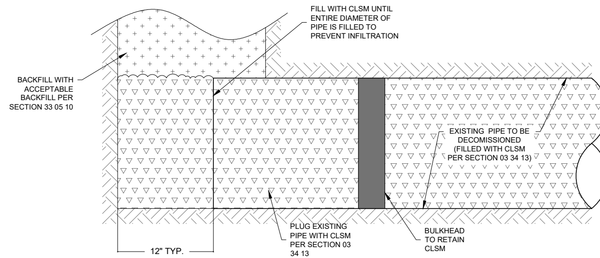
PIPE ABANDONMENT IN PLACE NOT TO SCALE
