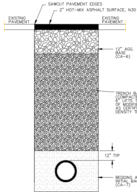
OPEN CUT TEMPORARY STREET RESTORATION (TEMPORARY PATCH, 2")
